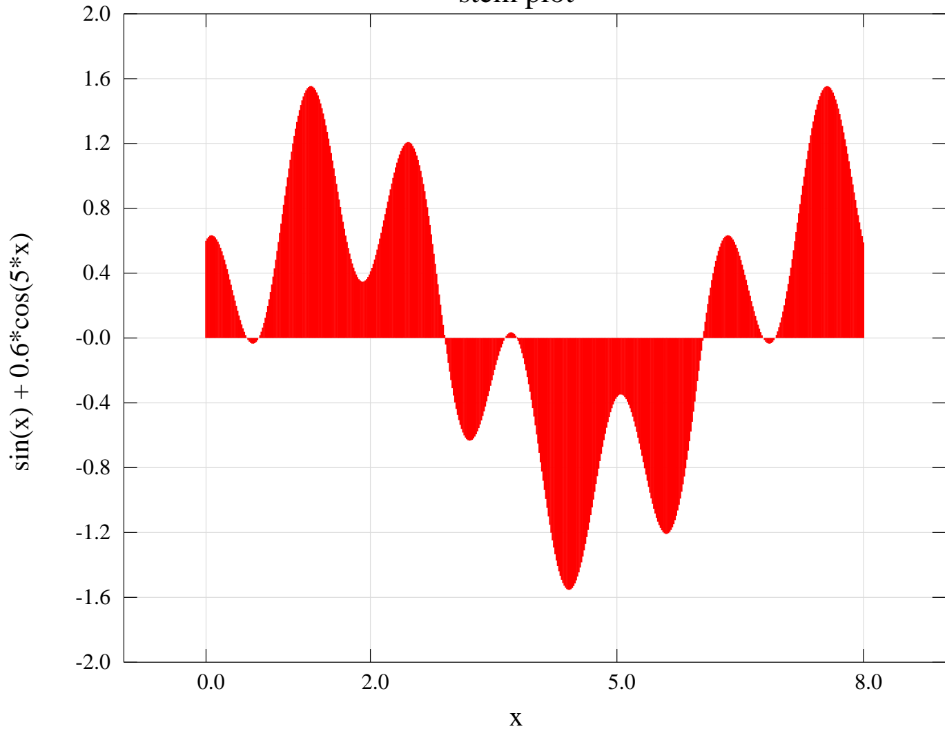
stem plot
